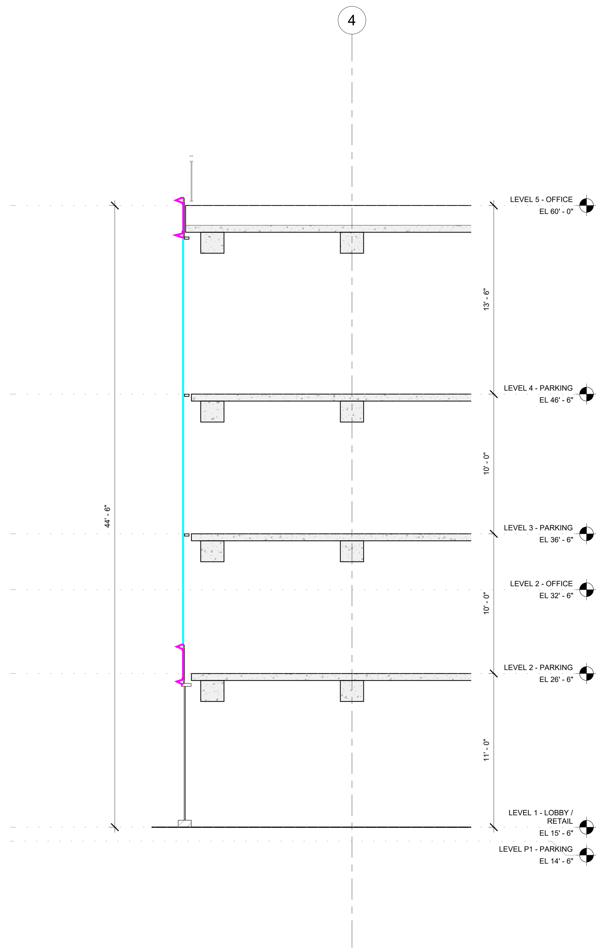
1 WALL SECTION 1/4" = 1'-0"
