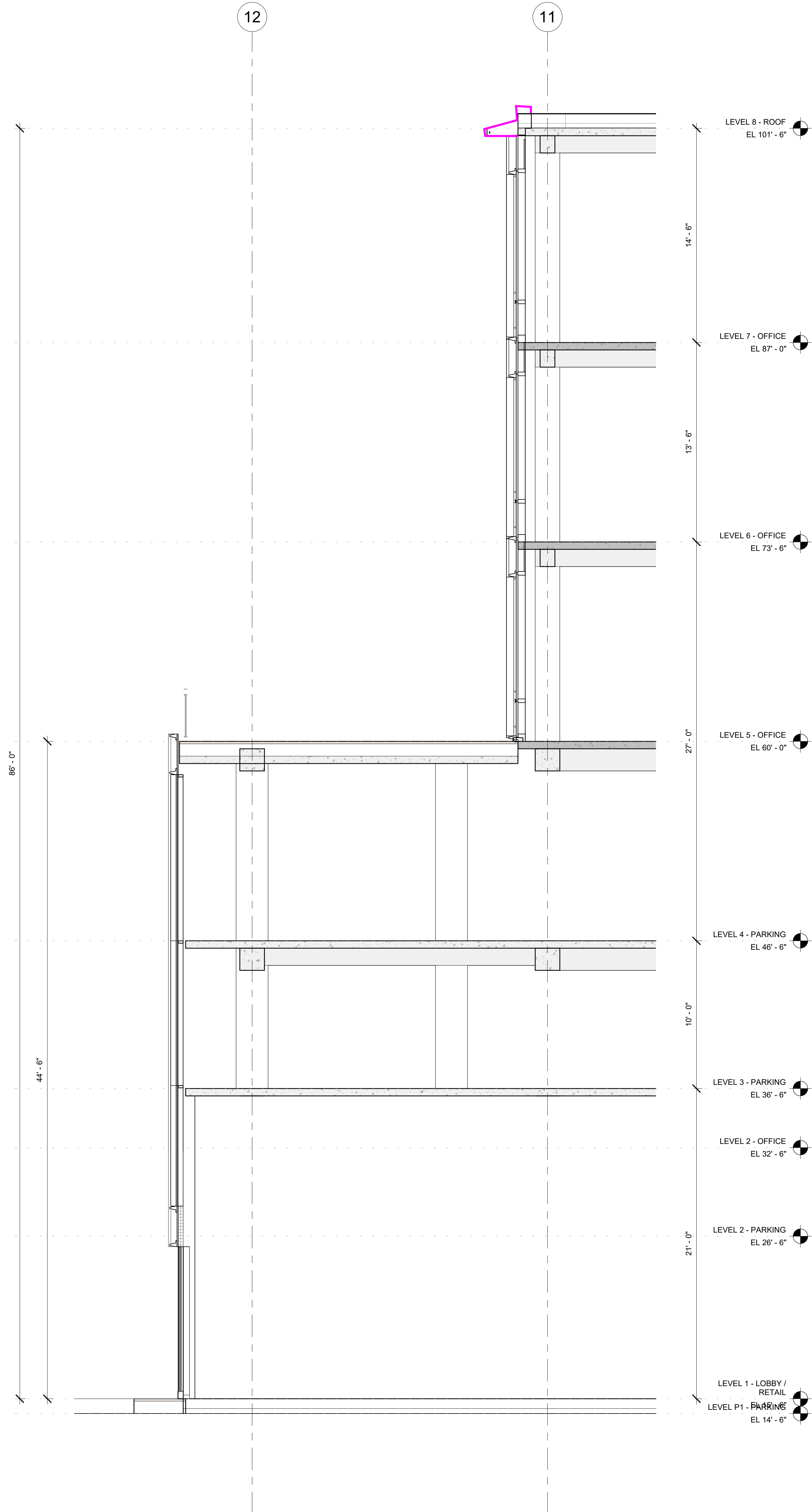
2 WALL SECTION 1/4" = 1'-0"
